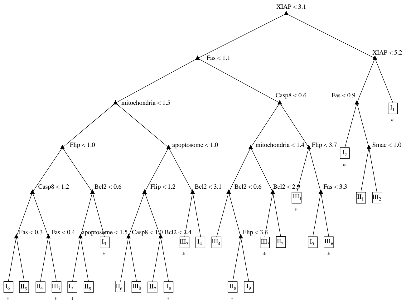
Figure 4. Decision tree model based on the Fas mechanistic model simulation data. The internal nodes have a triangle shape and the leaf nodes have a square shape. Roman numerals I, II and III for the leaf nodes correspond to the insensitive-response, medium sensitive-response and sensitive-response clusters, respectively. Subscript numbers for the leaf nodes, which are ordered from top to bottom, are used to identify each leaf node. The leaf nodes with over 66% prediction accuracy (in the training set) are marked with asterisks.
